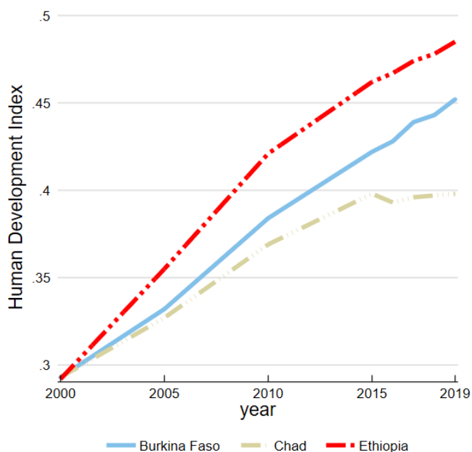
Figure 2: HDI trends for Ethiopia, Chad and Burkina Faso, 2000-2019
