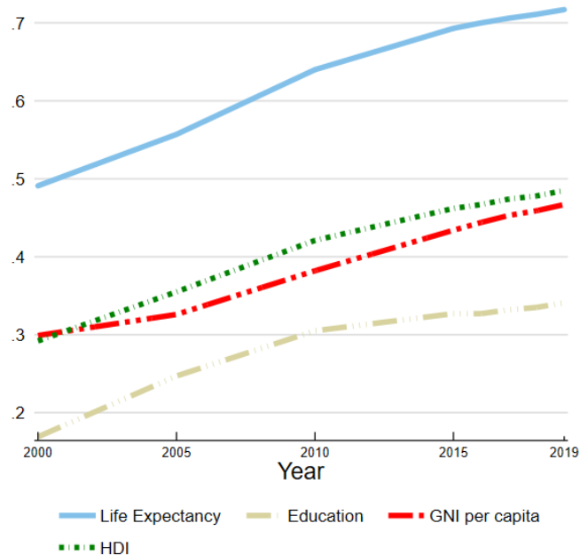
Figure 1: Trends in Ethiopia's HDI component indices 2000-2019
